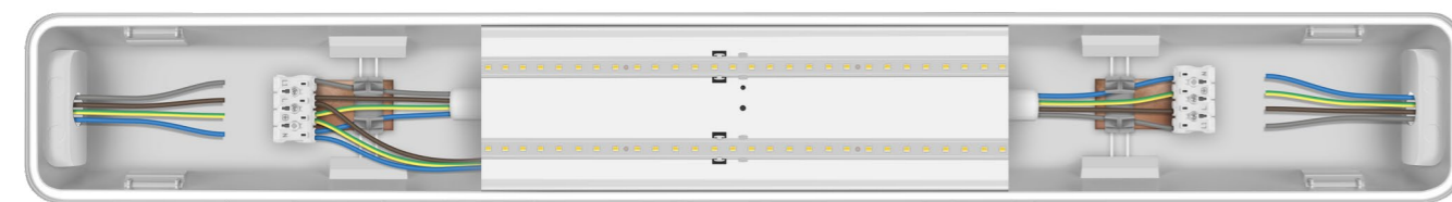
The loop-in/loop-out terminals make it possible to wire from fitting-to-fitting
