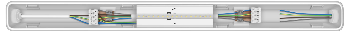
Standard - Equivalent Replacement for Single Fluorescent T8 Fittings
