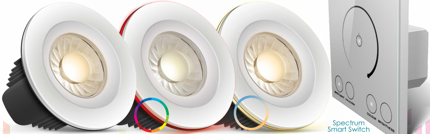
Spectrum Orion
